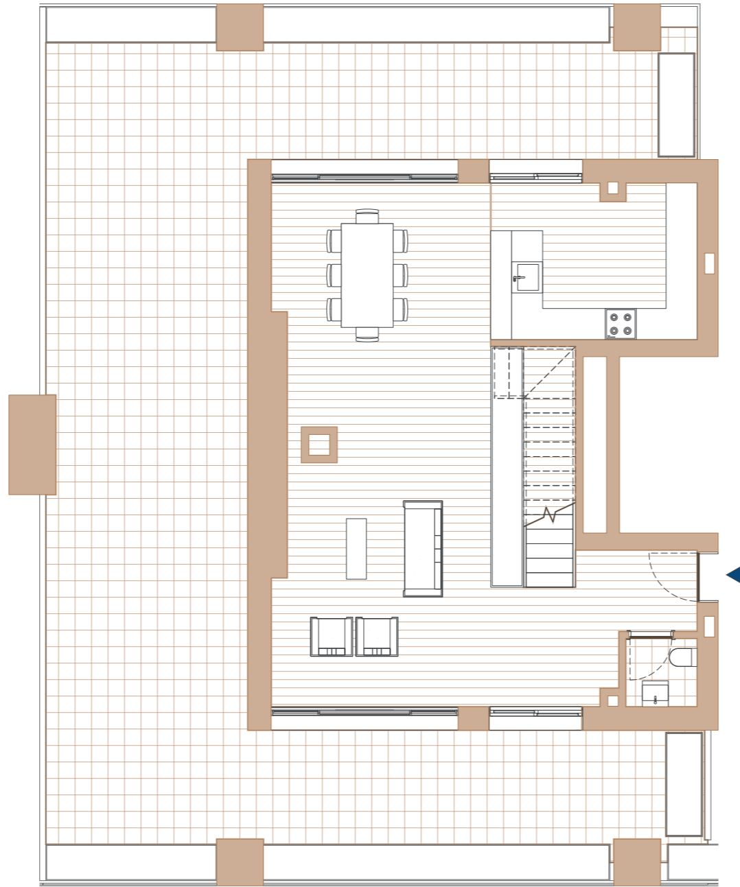
Piso Floor 2
